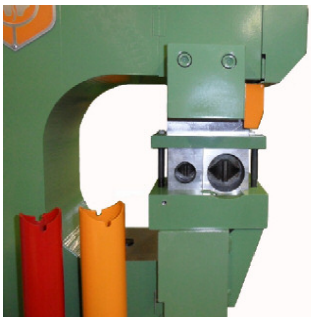
4-station pipe notching attachment, mounted on the punch unit. The finger protection has been removed for the picture.
