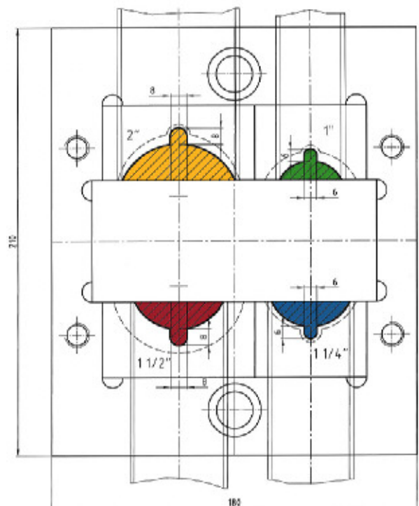
4-station pipe notching attachment, mounted on the punch unit. The finger protection has been removed for the picture.
