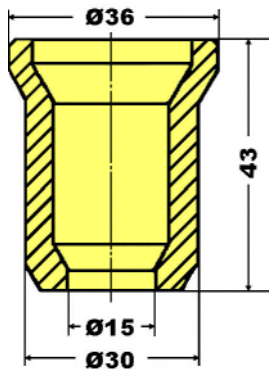
Reduceerhuls 30/15 10505 313 00 00
