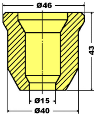
Reduceerhuls IV/I 10505 314 00 00
