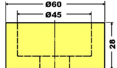
Reduceerinzet 60/45 10506 063 00 00
