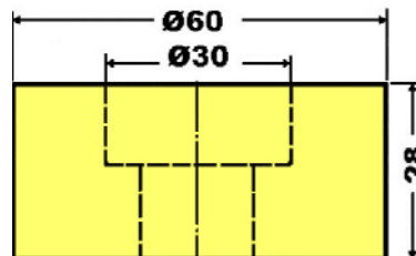
Reduceerinzet 60/30 10506 062 00 00
