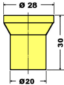
Reduceerhuls 10505 290 00 00
