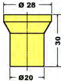
Stempelbeilage punch sleeve garniture de poinçon 10505 290 00 00
